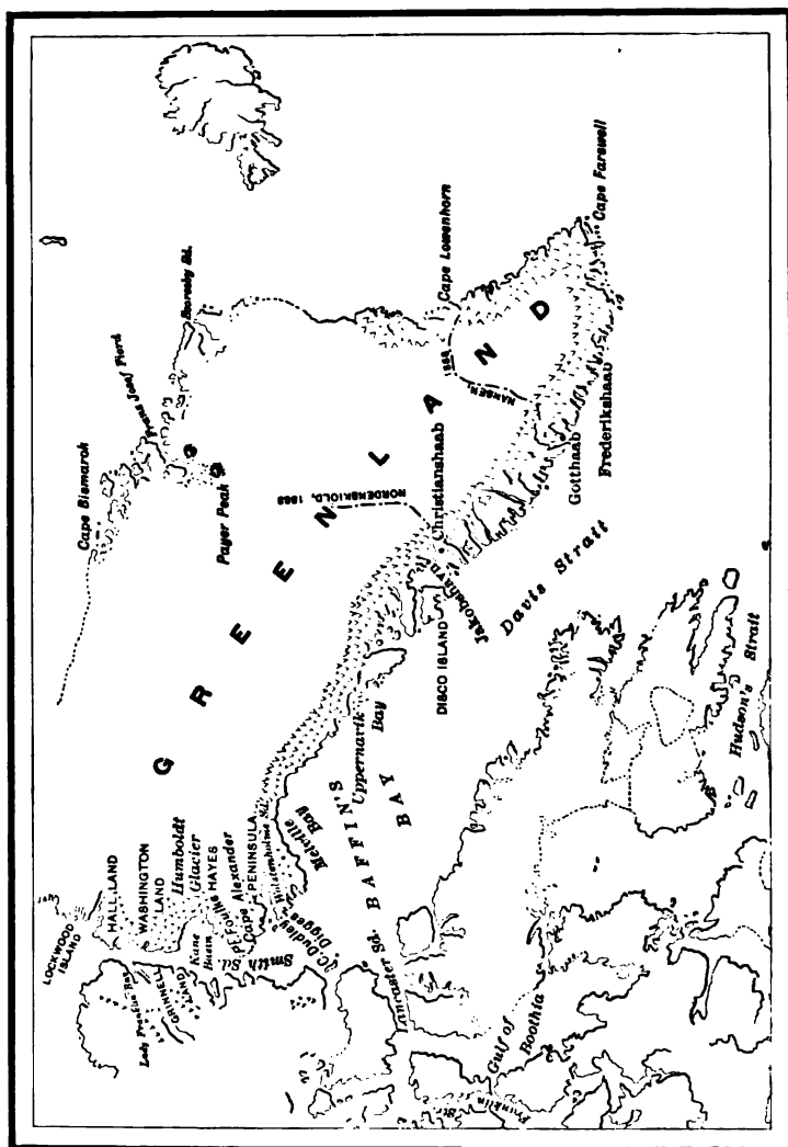
FIG. 29.—Map of Greenland. The arrow-points mark the margin of the ice-field.
